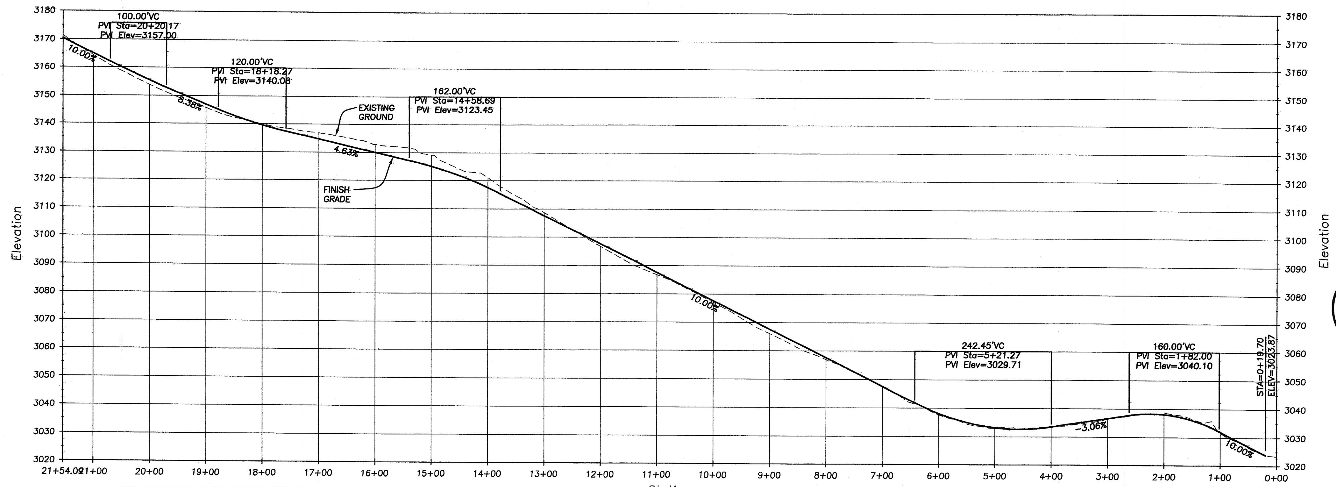
TIMBERLINE DRIVE PROFILE HORIZONTAL SCALE: 1"=100' VERTICAL SCALE: 1"=10'
