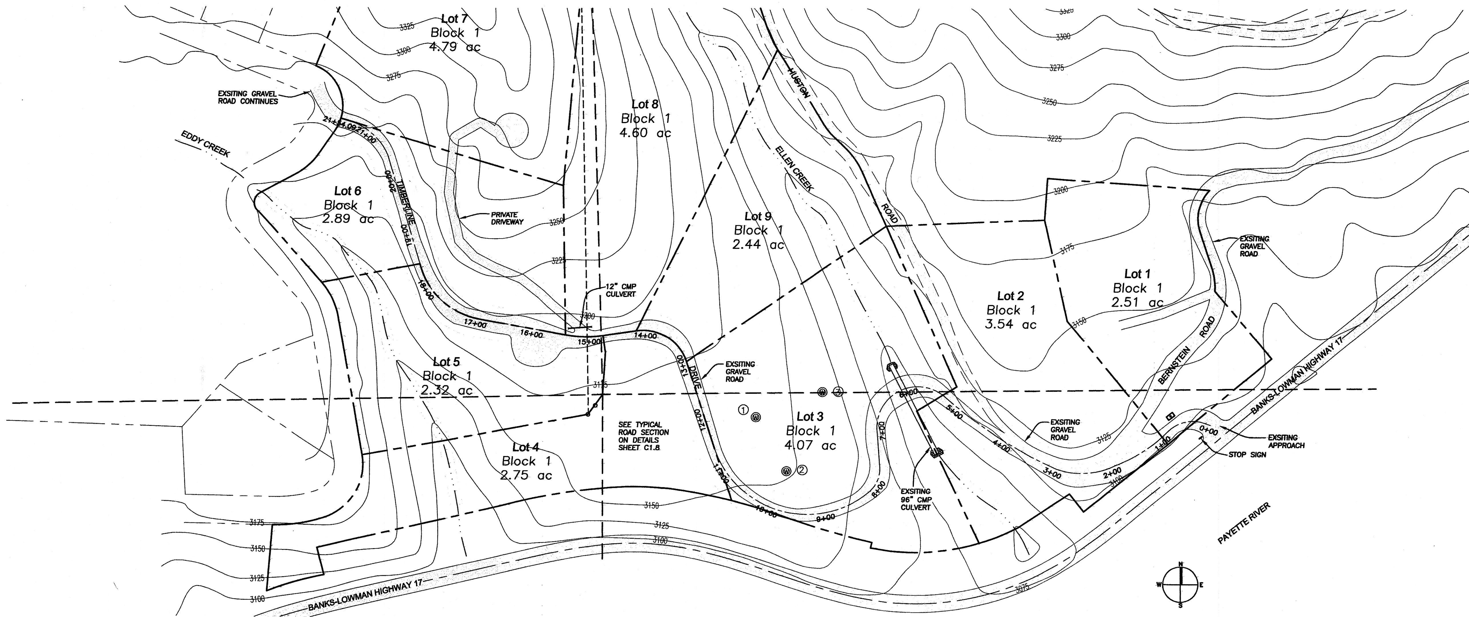
TIMBERLINE DRIVE PLAN SCALE: 1"=100'
